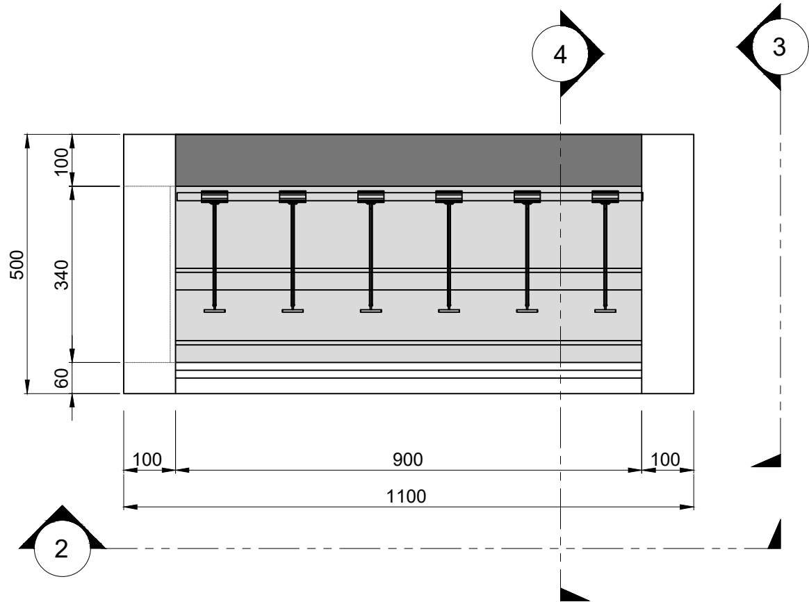
1 PLAN
